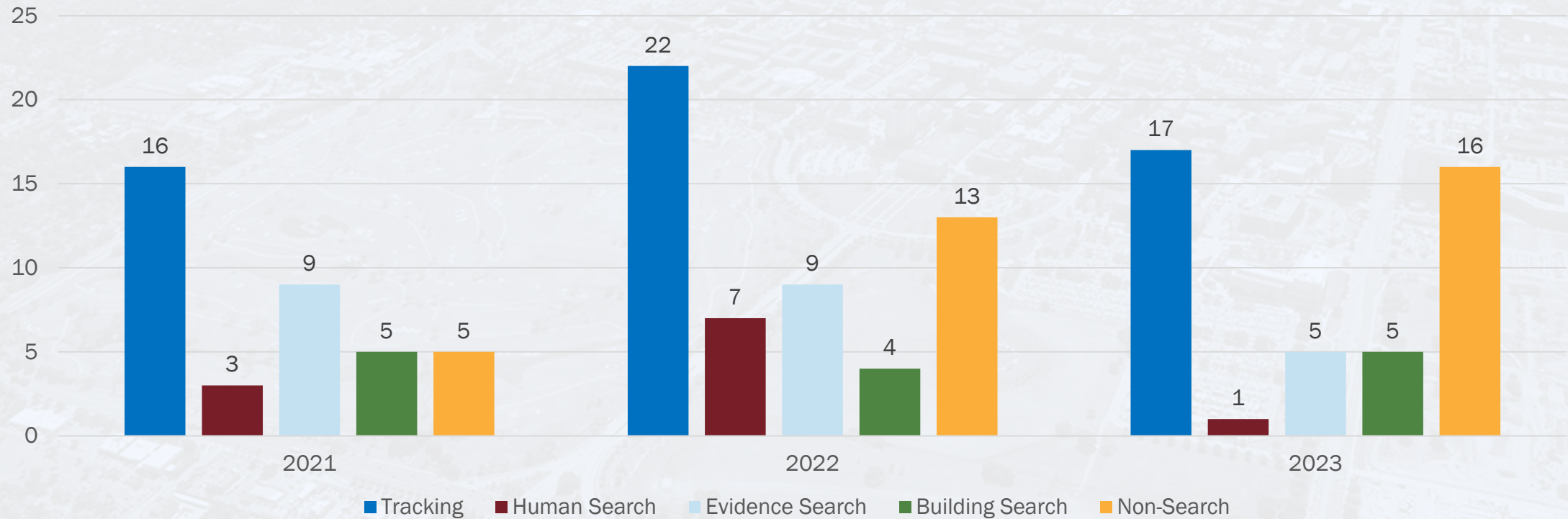
Patrol Deployments
